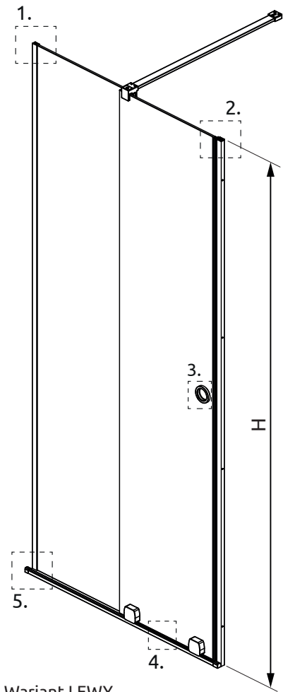
Wariant LEWY Variant L
